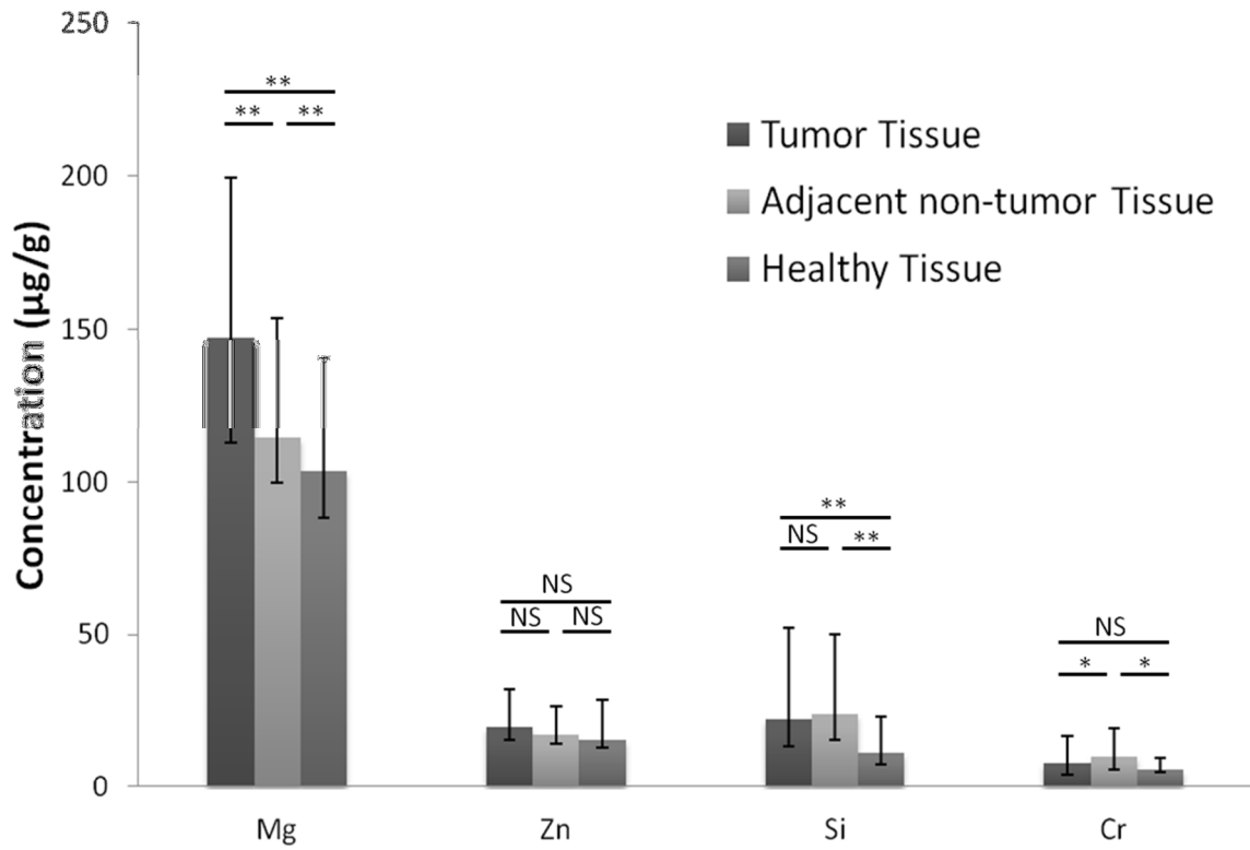
Figure 1: Median concentrations of Mg, Zn, Si and Cr expressed in \mu\text{g} of element per g of wet tissue (NS: not significant, *p < 0.05 , **p < 0.01 , Z-test, Wilcoxon test and Mann-Whitney test for independence)
