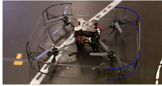
Fig. 2: Experimental Octocopter
