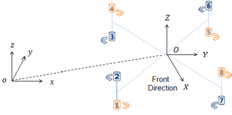
Fig. 1: The coaxial octorotor and the reference frames
