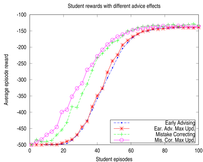
Fig. 8. Student's reward considering different heuristics with either informed-exploration or max-update (budget = 75; threshold for mistake correcting with informed exploration: 128; threshold for mistake correcting with max update: 140)
