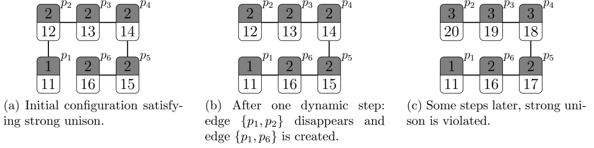
Figure 3: Example of execution when adding and removing one edge: \mu = 6 , \alpha = 7 , and \beta = 42 . The value of c - (resp. t -) variable is in the upper (resp. lower) part of the node.
