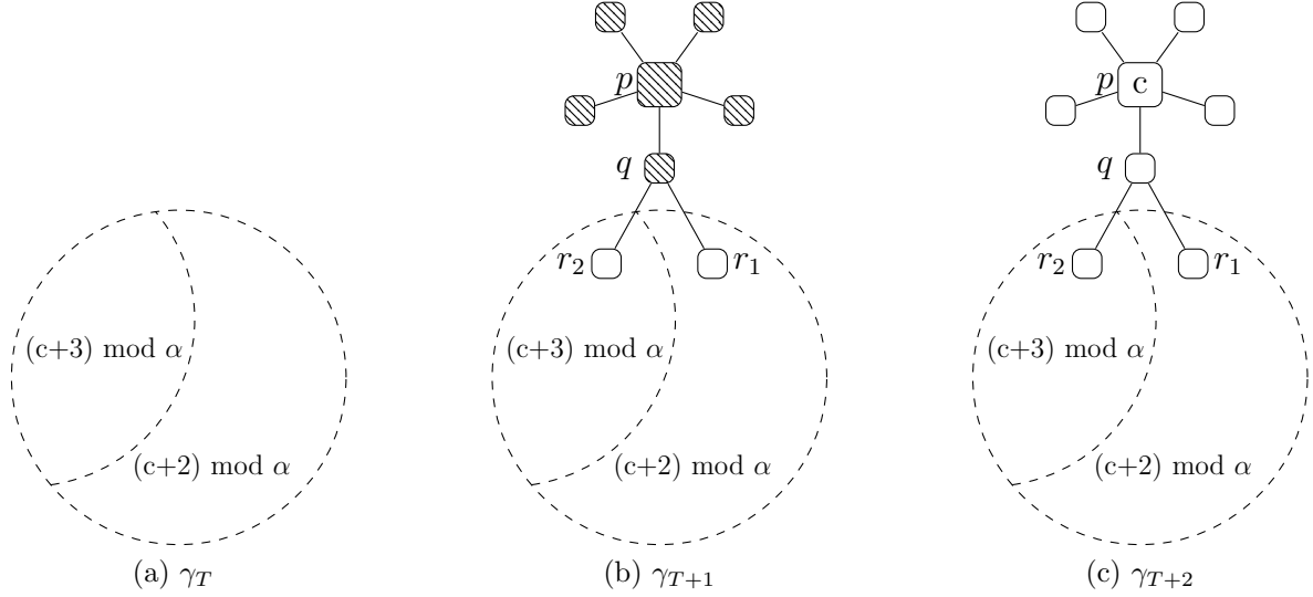
Figure 1: Execution e'' in the proof of Theorem 1. The hatched nodes are in New .
