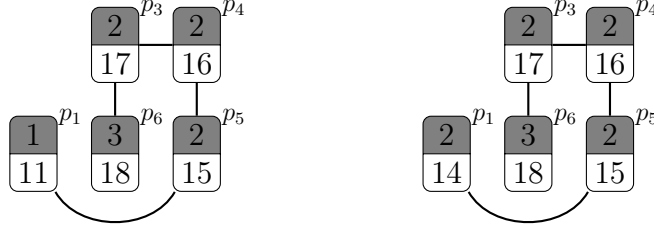
(d) After some steps, strong unison is not satisfied yet but weak unison is still satisfied.
