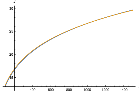
Fig. 3: exact (blue) and approximate (yellow) values for J(L) .
