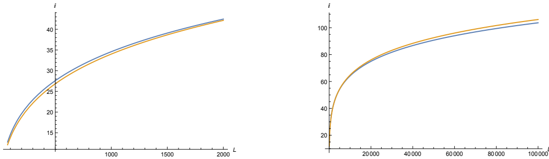
Fig. 5: comparison between the present calculation of I(L) (blue) and Jancovici's final refined estimate with A = 3.5 , I(L) \simeq (\ln 2L - \gamma_E - \frac{3}{2})^2 + 3.5 (yellow).
