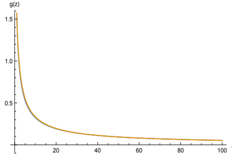
Fig. 2: exact (blue) and approximate (yellow) values for the integrand g(z) of J(L) .
