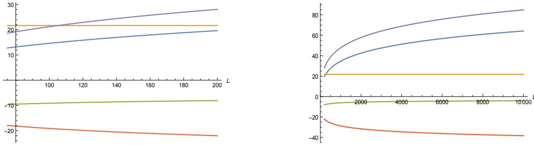
Fig. 4: contributions to the Demeur-Jancovici integral; constant term (yellow), inverse power (green), \ln (red), \ln^2 (violet), sum of all (blue).
