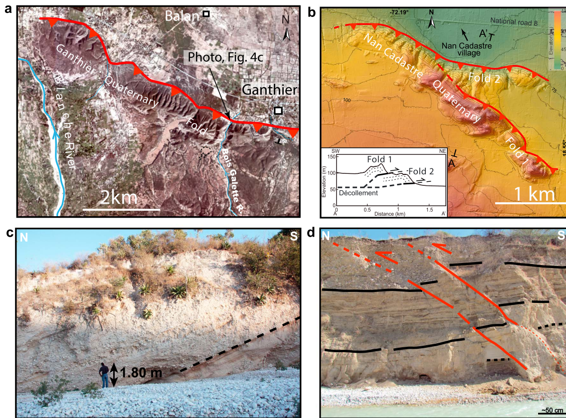
Figure 4. Active folding in the Cul-de-Sac-Enriquillo ramp basin. (a) Aerial photograph of the 8 km long Ganthier Quaternary fold. (b) Lidar topography of the Nan Cadastre Quaternary thrust folding. Inset: topographic profile AA' and possible interpretation at depth. (c) Field photograph along the eastern flank of the Bois Galette River (location in Figure 4a) showing the folded alluvial sediments of the Ganthier fold dipping \sim 30^\circ\text{N} . (d) Field photograph and interpretation of the 50 \pm 15^\circ southward dipping Dumay thrusts (in red) exposed in cross section on the eastern bank of the Rivière Grise (location in Figure 2a). The fault offsets by several tens of centimeters Quaternary sediments (lacustrine and conglomerates) incised by the river.
