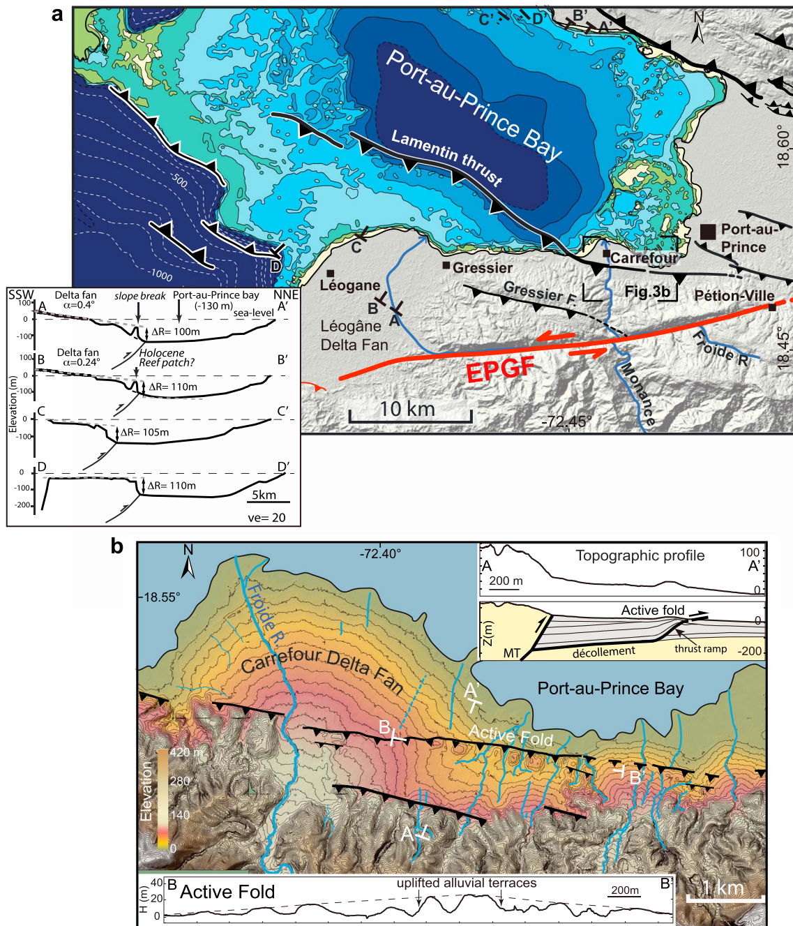
Figure 3. (a) Active faulting in the 2010 earthquake epicentral area. Active faults, symbols, topography, and bathymetry as in Figure 2a. Location of Figure 3b is indicated. SSW-NNE topographic profiles are shown in the inset. \Delta R : fault throw at the seafloor. Vertical exaggeration (VE): 20X; \alpha : slope of the Léogâne delta fan. (b) The Lamentin thrust in Carrefour. Topography from lidar data (contours at 5 m vertical interval). Rivers in blue, with thicker traces for larger ones. Inset in the lower left corner: topographic profile BB' along of the Lamentin fold crest (VE: 5X). Inset in the upper right corner: topographic profile AA' perpendicular to the Lamentin thrust system (VE: 2.5X) and the most plausible geometry of the thrusts (with no vertical exaggeration). In yellow: upper Miocene limestone; in grey: Quaternary conglomerates. MT: main thrust. The width of the fold and the slope of the fan surface constrain the rooting depth of the emergent ramp to the décollement [e.g., Meyer et al. , 1998].
