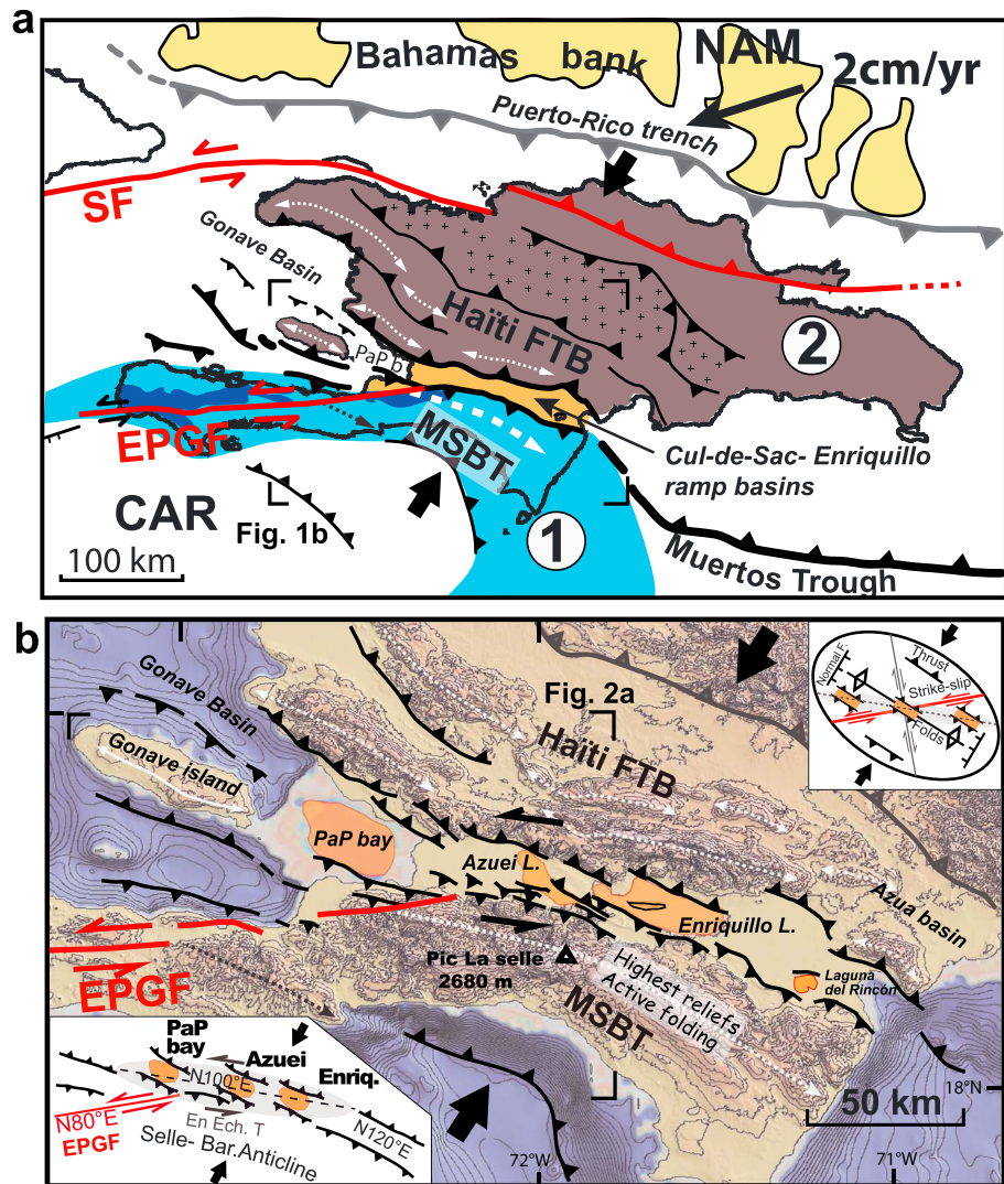
Figure 1. Tectonic setting and active faulting in Haiti. (a) Major anticlines (lines with arrows, dashed white: growing and grey: older), active thrusts (black), and strike-slip faults (EPGF and SF: in red) from this study [Mann et al., 1995; Pubellier et al., 2000; Mauffret and Leroy, 1997; Granja Bruña et al., 2014]. Blue (1): rigid Beata oceanic crust block. Dark purples: toleitic complex oceanic crust outcrops. Orange: Cul-de-Sac and Enriquillo (CSE) ramp basins; brown (2): Hispaniola volcanic arc. Black crosses: metamorphic Cretaceous basement; yellow: rigid Bahamas bank. Haiti FTB: Haiti fold and thrust belt. Grey line: trench. Double black arrows: regional compression deduced from mean orientations of folds and thrusts. (b) Active faulting in southern Haiti. Topography and bathymetry (contours each 200 m) from Global Multi-Resolution Topography (GMRT) synthesis ( http://www.geomapapp.org ). Faults, folds, and symbols as in Figure 1a. Simple red and black arrows: strike-slip motion. In orange: push-down troughs of Port-au-Prince Bay and Azuei and Enriquillo Lakes in the CSE ramp basin. Inset (bottom left): fault geometry and kinematics. Grey ellipse: zone with en echelon troughs in N100°E direction. Inset (top right): simplified strain ellipse in southern Haiti.
