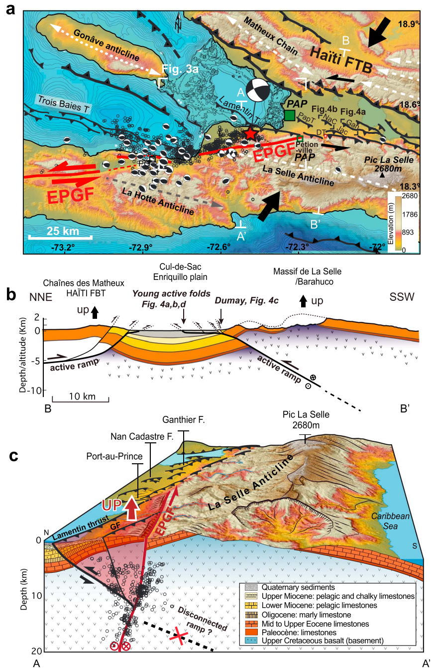
Figure 2. (a) Active faulting and seismicity in the southeastern part of Haiti. Topography and bathymetry (contours each 100 m), from Advanced Spaceborne Thermal Emission and Reflection ( http://asterweb.jpl.nasa.gov/ ) and Shuttle Radar Topography Mission 30+ ( http://www2.jpl.nasa.gov/srtm/ ), respectively, and the 1:25000 bathymetric chart of the Hydrographic and Oceanographic Department of the French Navy (contours at -2 , -5 , -10 , -20 , -30 , -50 , -100 , and -130 m) in the Port-au-Prince Bay. Faults, folds, and symbols as in Figure 1. Red star: 2010 main shock epicenter from Mercier de Lépinay et al. [2011] with the centroid moment tensor from Harvard University ( http://www.globalcmt.org/ ); seismicity from Douilly et al. [2013], and focal mechanisms from Nettles and Hjörleifsdóttir [2010]. Location of Figure 3a is indicated. PAP, Port-au-Prince. Folds in CSE ramp basin with locations of Figures 4a and 4b are indicated: PaPT: Port-au-Prince thrust; DT: Dumay thrust; NaC: Nan Cadastre thrust (see Figure 4b); Jac: Jacquet thrust; Gan: Ganthier thrust (see Figure 4a). Red and white star near DT: location of Figure 4d. (b) NNE-SSW geological cross section across the Cul-de-Sac-Enriquillo plain. Geology from www.bme.gov.ht and Mann et al. [1991b] (supporting information Figure S5) with colors of units as in Figure 2c. Profile location shown in Figure 2a; topography as in Figure 1. No vertical exaggeration. (c) Three-dimensional block diagram showing the geology, the aftershocks [from Douilly et al. , 2013], and the fault system along a N-S cross section (location in Figure 2a). The block highlighted in red is uplifting in between the LT and the EPGF.
