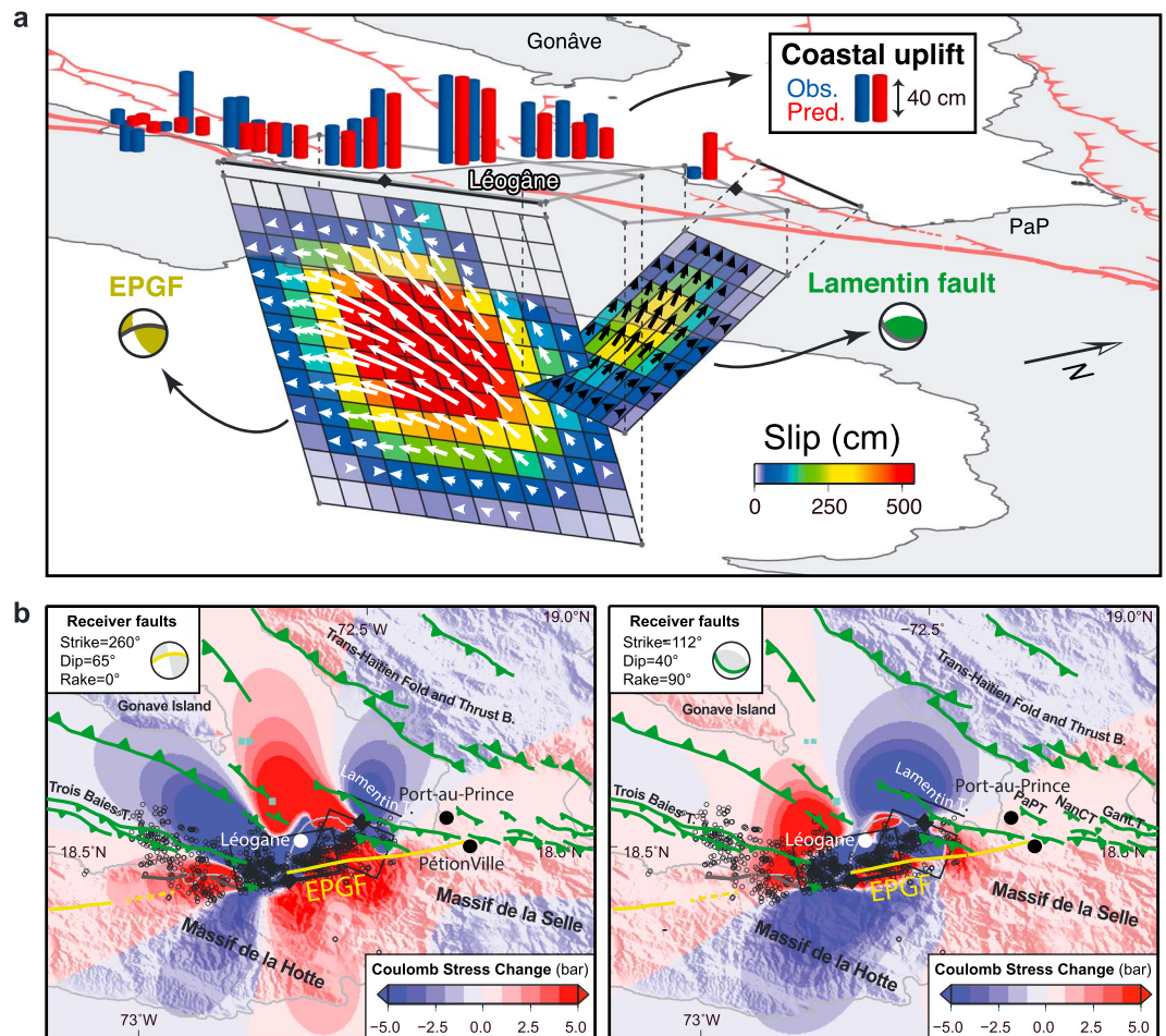
Figure 5. New static slip model for the 2010 Haiti earthquake and induced Coulomb stress changes. (a) Axonometric view from SE showing the slip distribution on two faults (EPGF and LT) determined by modeling geodetic data (GPS and interferometry) and coastal uplift values recorded by coral (see supporting information). Arrows (white for EPGF and black for LT) indicate the motion of the hanging wall with respect to the footwall. Land surfaces in grey. Red lines: active faults. Blue bars: coastal uplift measured by using corals from Hayes et al. [2010]. Red bars: uplift predicted by our model. Focal mechanisms indicated the EPGF (dark yellow) and Lamentin fault (green) geometry. (b) Coulomb stress changes induced by the slip model we determined, in map view at 7.5 km depth. Black rectangles: modeled faults. Epicentral locations of aftershocks from Douilly et al. [2013]. Insets in the upper left corners: parameters of the receiver faults used for the Coulomb stress calculation. Calculated for receiver faults having the same geometry as the strike-slip EPGF (dark yellow lines) and as the Lamentin thrust (dark green lines), respectively (Figure 5b, left and right).
