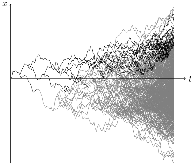
Figure 1 – Simulation of a BBM starting with a single particle at 0 and of the coupled L -BBM with L = 3 between times 0 and 7. Particles in black belong to the L -BBM and particles in grey belong only to the BBM without selection and not to the L -BBM. Note that quickly some particles killed by selection have descendants with a better fitness value than the particles of the L -BBM.
