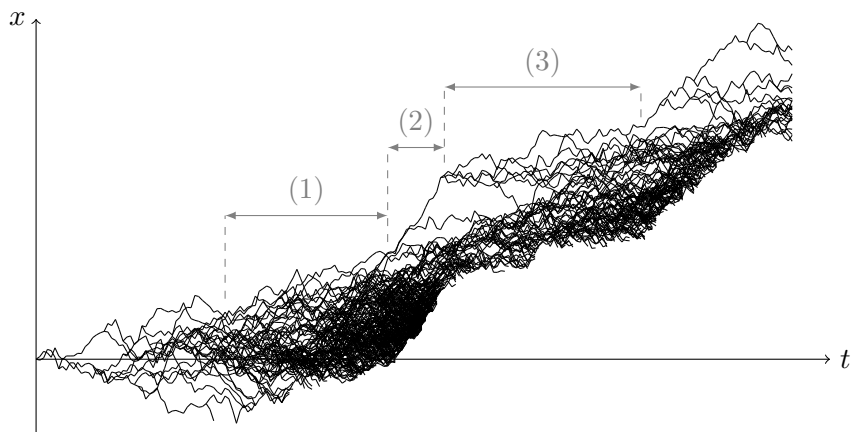
Figure 2 – Simulation between times 0 and 10 of an L -BBM with L = 5 starting with a single particle at 0. During the period (1), \max X^L grows slowly so the number of particles becomes very large. Among all these particles, there is one that goes up very fast during the period (2) and it reduces drastically the population. Therefore, after that, during period (3), \max X^L grows once again slowly, involving an increase of the population size.
