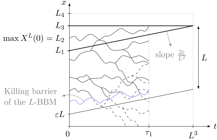
Figure 6 – Representation of the coupled systems X^L (full line) and \tilde{X}^{L_4, L_3} (dashed line) between times 0 and \tau_1 , starting with the highest particle at L_2 , on the event A_0 . Until time \tau_1 , the killing barrier of X^L (drawn in blue) stays above the straight line t \mapsto \varepsilon L + \frac{2\varepsilon}{L^2}t so above 0.
