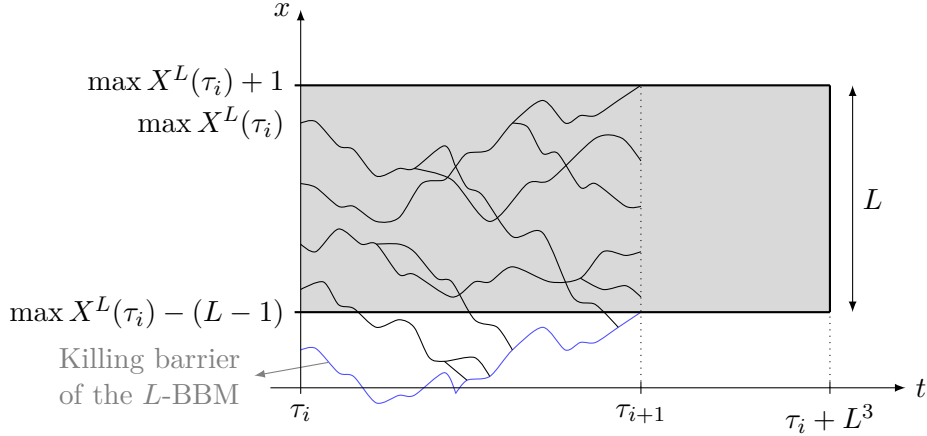
Figure 3 – Representation of a L -BBM between times \tau_i and \tau_{i+1} . By definition, \tau_{i+1} is the time where t \mapsto \max X^L(t) leaves the gray area. We are here on the event A_i^c because t \mapsto \max X^L(t) leaves the area from above. Note that the killing barrier of X^L (drawn in blue) stays below \max X^L(\tau_i) - (L - 1) .
