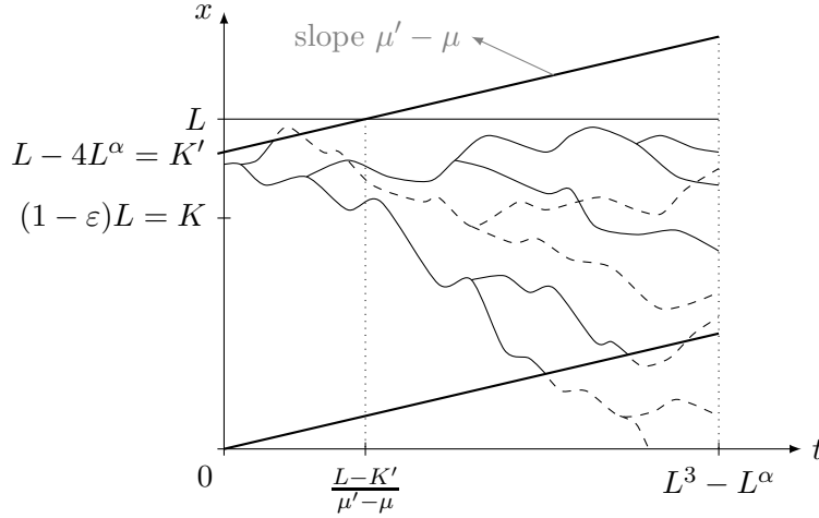
Figure 4 – Representation of the coupled systems \bar{X} (full line) and \tilde{X}^{K,L} (dashed line) starting with a single initial particle at K' - 1 , on the event C'_0 . The two thick straight lines of slope \mu' - \mu are the killing barriers that define \bar{X} .
