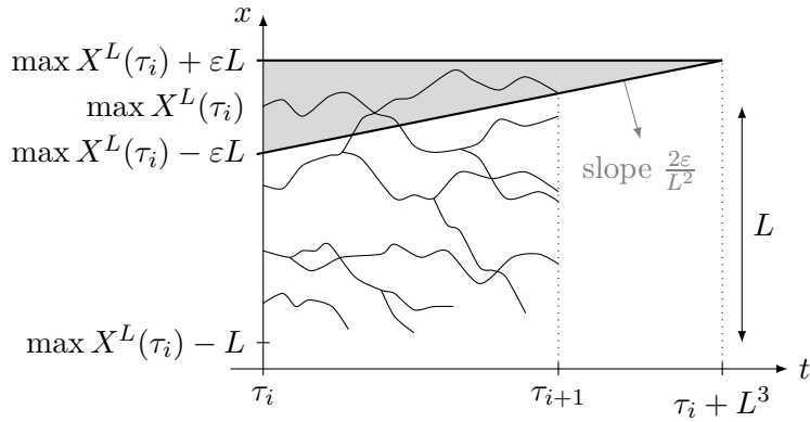
Figure 5 – Representation of a L -BBM between times \tau_i and \tau_{i+1} . By definition, \tau_{i+1} is the time where t \mapsto \max X^L(t) leaves the gray area. The two thick straight lines that delimit the gray area intersect at time \tau_i + L^3 . We are here on the event A_i^c because t \mapsto \max X^L(t) leaves the area from below.
