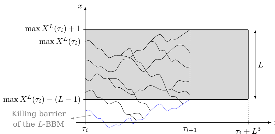
Figure 3: Representation of a L -BBM between times \tau_i and \tau_{i+1} . By definition, \tau_{i+1} is the time where t \mapsto \max X^L(t) leaves the gray area. We are here on the event A_i^c because t \mapsto \max X^L(t) leaves the area from above. Note that the killing barrier of X^L (drawn in blue) stays below \max X^L(\tau_i) - (L - 1) .
