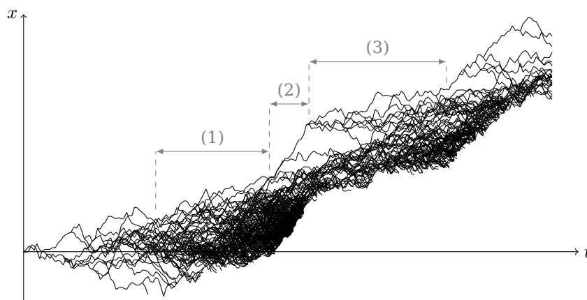
Figure 2: Simulation between times 0 and 10 of an L -BBM with L = 5 starting with a single particle at 0. During the period (1), \max X^L grows slowly so the number of particles becomes very large. Among all these particles, there is one that goes up very fast during the period (2) and it reduces drastically the population. Therefore, after that, during period (3), \max X^L grows once again slowly, involving an increase of the population size.
