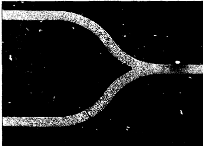
Figure 8: SEM micrograph of part of a Mach-Zehnder interferometer.
