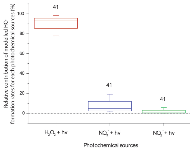
Figure 6. Distribution of relative contributions of modelled HO formation rates for each photochemical source ( \text{H}_2\text{O}_2 , \text{NO}_3^- and \text{NO}_2^- photolysis) for all cloud water samples. Model outputs are obtained from the sensitivity test in which the iron chemistry is not considered, and new photolysis rate constants from experimental measurements are implemented in the model. The number of samples analysed is indicated above each boxplot. The bottom and top lines correspond to the 25th and 75th percentiles, respectively. The full line represents the median values. The ends of the whiskers are the 10th and 90th percentiles.
