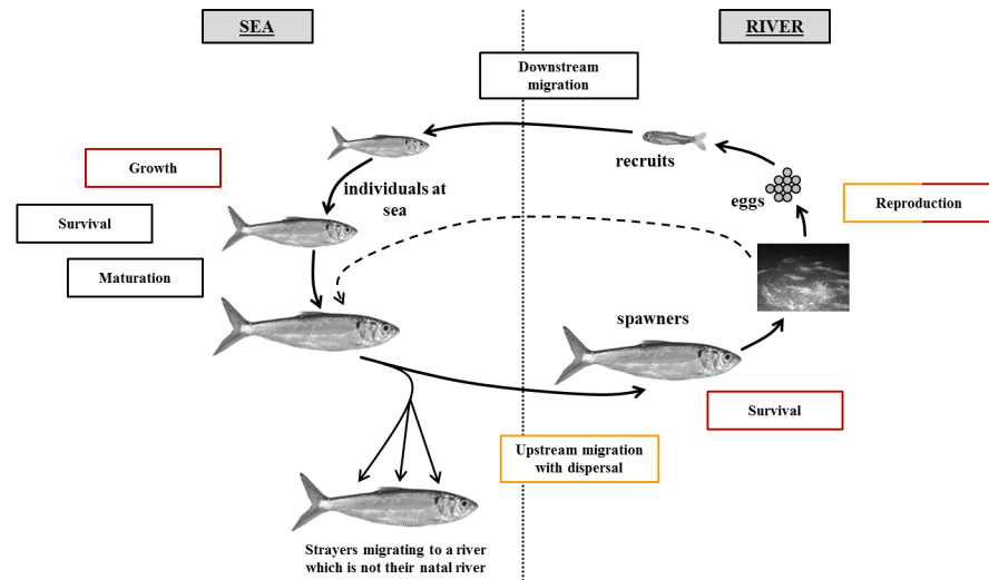
Fig 1. Conceptual diagram of the life cycle of anadromous species (adjusted to allis shad) represented in the GR3D model. Red boxes depicted the processes in GR3D that were influenced by temperature and orange boxes the ones that were linked to the surface area of the drainage basin. The figure was adapted from [26] for illustrative purpose only.
