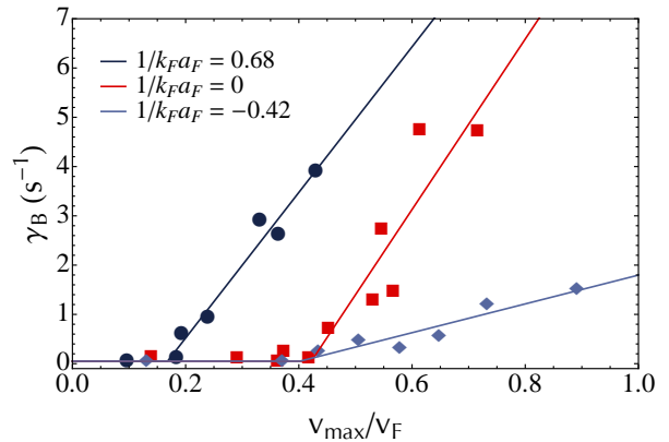
FIG. 2: Damping rate of the center of mass oscillations versus maximal relative velocity in the BEC-BCS crossover in unit of the Fermi velocity v_F . Dark blue dots: BEC side (780 G) 1/k_F a_F = 0.68 , red squares: unitarity (832.2 G) 1/k_F a_F = 0 , light blue diamonds: BCS side (880 G) 1/k_F a_F = -0.42 . Power law fits with thresholds provide the critical velocity (solid lines).
