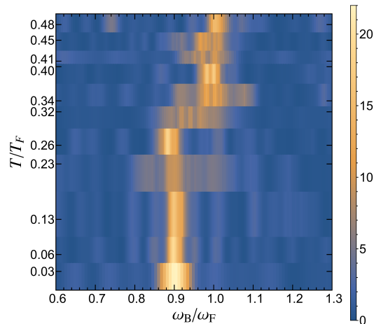
FIG. 4: Power spectrum of the oscillations for different temperatures, obtained using the Lomb-Scargle algorithm of the center-of-mass displacement. Above T \approx T_{c,B} \approx 0.34 T_F > T_{c,F} , oscillations of the Bose and Fermi clouds become locked together at \omega_F . A value of 10 for the power represents typically a significance of 0.002 [28].
