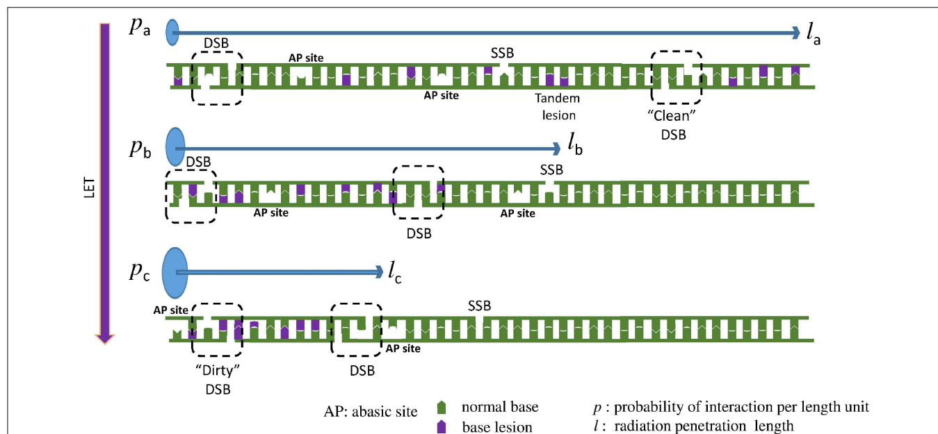
FIGURE 4 | When LET increases the DNA lesions are denser
