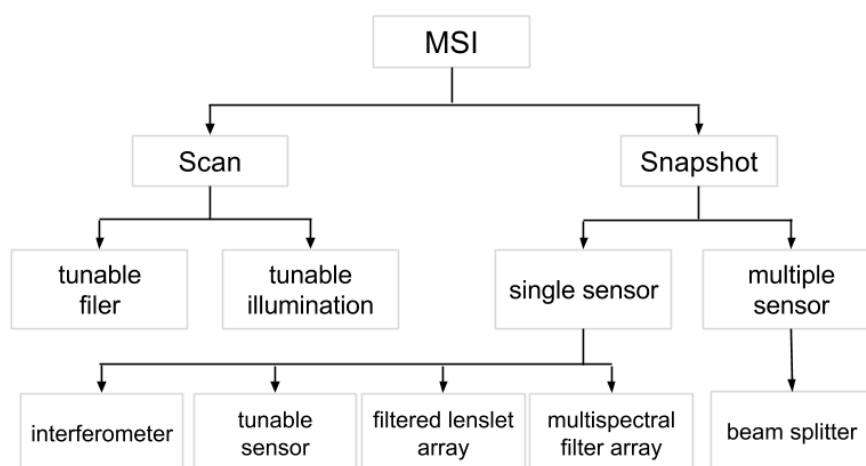
Figure 2. Classification tree of the main methods for multispectral capturing.
