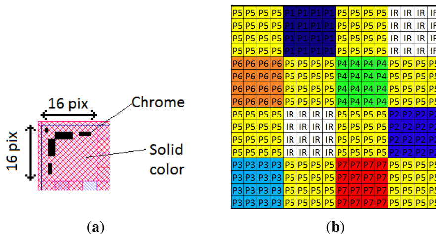
Figure 12. One alignment matrix (a), in the top left corner of the filter array; (b) Each filter covers 4 \times 4 pixels of the sensor.
