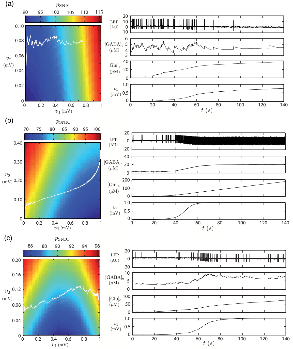
Figure 8: Alteration of astrocytic glutamate uptake (a) lessening the excitability, (b) resulting in sustained hyperexcitability, (c) resulting in transient hyperexcitability. In each case, the colormap on the left displays the value of p_{\text{SNIC}} in (v_1, v_2) plane, and the time series on the right correspond to LFP, [\text{GABA}]_e , [\text{Glu}]_e and v_1 = m_G^I \mathcal{S}([\text{Glu}]_e, v_G, r_G) . The white curves on the colormap are the traces of (m_G^I \mathcal{S}([\text{Glu}]_e, v_G, r_G), m_\gamma \mathcal{S}([\text{GABA}]_e, v_\gamma, r_\gamma)) along the associated orbits of the model. At t = 20\text{s} , we alter the glutamate astrocytic uptake by setting V_G^{\text{ae}} = 0 . The three cases are obtained with : (a) \frac{m_G^P}{m_G^I} = 1.7 , (b) \frac{m_G^P}{m_G^I} = 3.2 , (c) \frac{m_G^P}{m_G^I} = 2.43 . All other parameters are the same in the three cases and given in Table 1.
