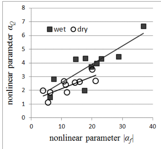
Figure 5: Correlation between the nonlinear elastic coefficient \alpha_f and the nonlinear dissipative coefficient \alpha_Q measured in dry and wet cortical bone specimens.
