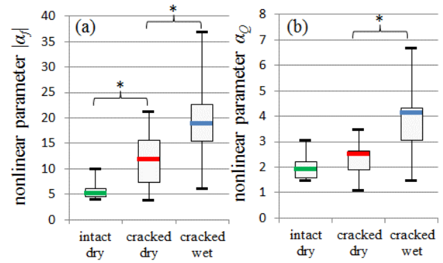
Figure 4 : Nonlinear elastic \alpha_f (a) and dissipative \alpha_Q (b) before and after crack propagation, measured in dry and wet conditions. For the sake of clarity, the two outliers (#1 and #8) are not represented.
