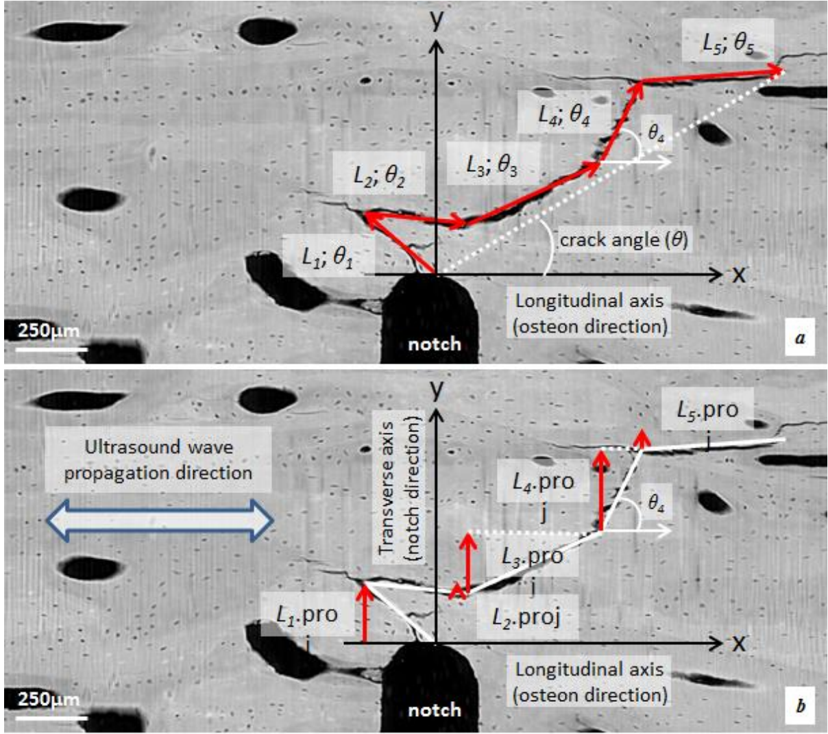
Figure 3: (a) Decomposition of the main crack into 5 vectors with lengths L_n and angles \theta_n . The crack length Cr.Le = L_1 + L_2 + L_3 + L_4 + L_5 . The mean crack angle is estimated in a coordinate system composed by the osteon direction (x axis) and the notch direction (y axis). It corresponds to the vector orientation between both extremities of the main crack. (b) The orthogonal projection of the main crack on the transverse axis corresponds to the sum of the 5 vectors projected on the same axis. Cr.Le.Proj = L_{1.proj} + L_{2.proj} + L_{3.proj} + L_{4.proj} + L_{5.proj} (with L_n.proj = L_n * \sin(\theta_n) ).
