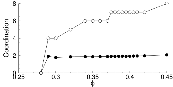
FIG. 3. Average (●) and maximum (○) coordination number in spanning clusters as a function of volume fraction ( L=20a ).
