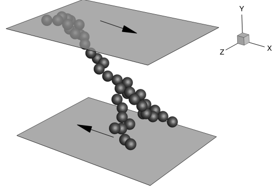
FIG. 2. A spanning cluster in a sheared bounded suspension ( \phi=0.32 ; L=30a ). Only particles belonging to spanning cluster are represented.
