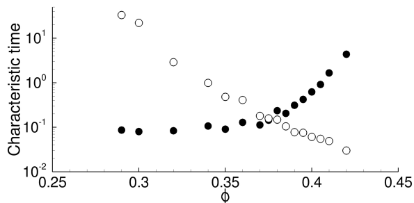
FIG. 4. Characteristic spanning times \langle\tau_s\rangle (●) and waiting times \langle\tau_w\rangle (○) as a function of volume fraction ( L=20a ; \phi_*=0.29 ). Times are rescaled by the inverse shear rate \dot{\gamma}^{-1} .
