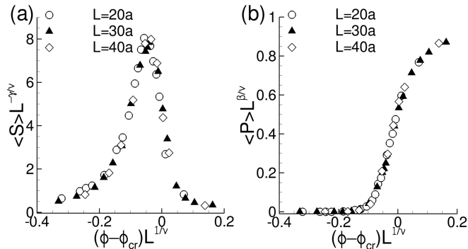
FIG. 5. Rescaled mean cluster size \langle S \rangle L^{-\gamma/\nu} (a) and rescaled strength \langle P \rangle L^{\beta/\nu} (b) as a function of (\phi - \phi_{cr}) L^{1/\nu} . The best data collapse is obtained for \phi_{cr} = 0.415 , \gamma = 1.91 , \nu = 1.02 and \beta = 0.18 . Scales are arbitrary since they depend on L (here, L is dimensional with a = 0.1 ).
