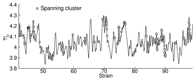
FIG. 6. Suspension relative viscosity \eta^r as a function of strain ( \phi = 0.34 , L = 20a ). A gray circle marks the presence of at least one spanning cluster.
