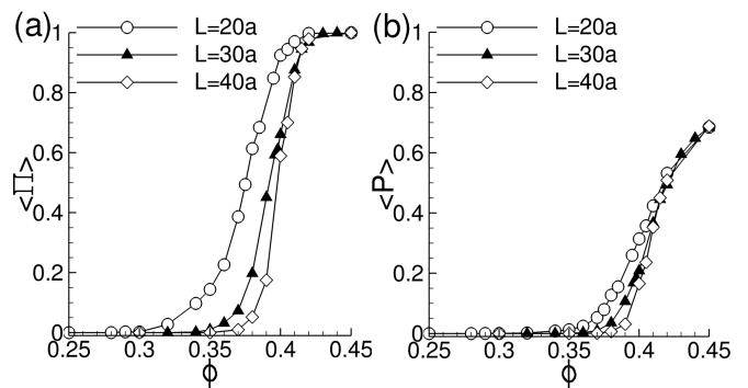
FIG. 1. Spanning probability \langle \Pi \rangle (a) and spanning strength \langle P \rangle (b) as a function of volume fraction \phi for different system sizes L .
