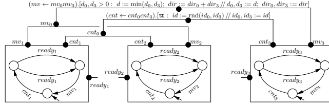
Figure 5: Leader/follower example with three atomic components
