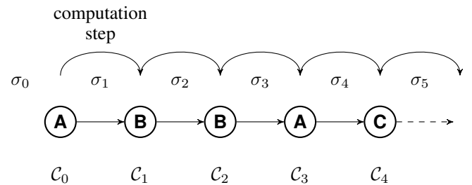
Fig. 2: Execution of a statistical deterministic Büchi automaton
