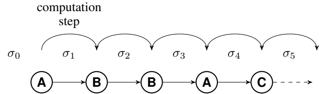
Fig. 1: Execution of a deterministic Büchi automaton
