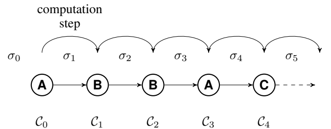
Fig. 2: Execution of a statistical deterministic Büchi automaton
