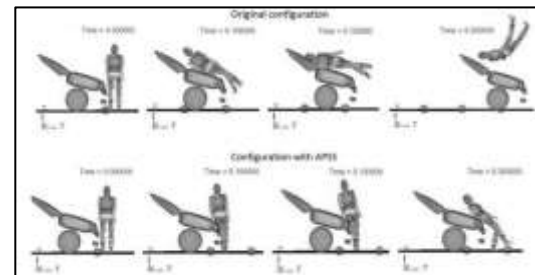
Figure 2 Crash simulation with and without APSS
