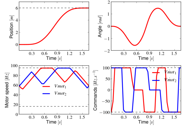
Fig. 2: Trajectories for the time optimal problem solved on the quadrotor system.
