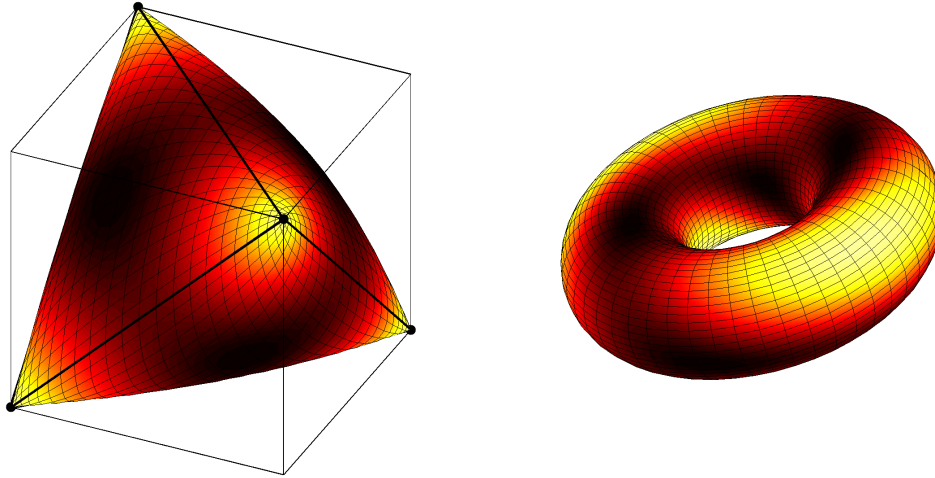
Figure 1: (Left) For m = 3, d = 1 , the set \mathcal{C} (2) contains all positive semidefinite matrices of the form X = [1, a, b; a, 1, c; b, c, 1] . It is here represented in coordinates (a, b, c) . The interior of the shell contains the rank-3 matrices; the four extreme points (black dots) are the rank-1 matrices; and the remainder of the boundary is the (smooth) set of rank-2 matrices. That smooth geometry breaks down at the rank-1 matrices. Note that for d > 1 , extreme points of rank d are no longer isolated. (Right) For m = 3, d = 1, p = 2 , the set \text{St}(d, p)^m (1) parameterizes the matrices of rank at most 2 in \mathcal{C} (redundantly). In this case, \text{St}(d, p)^m corresponds to a product of three circles in 2D: Y = [\cos \alpha_1, \sin \alpha_1; \cos \alpha_2, \sin \alpha_2; \cos \alpha_3, \sin \alpha_3] \in \text{St}(d, p)^m . One of these degrees of freedom is redundant, because the factorization of X \in \mathcal{C} as YY^\top is not unique. The figure represents the remaining degrees of freedom after fixing \alpha_1 = 0 . Notice how accepting the redundancy in the parameterization allows for a smooth representation of the nonsmooth set of bounded rank matrices in \mathcal{C} . Color codes for \|X\|_F = \|YY^\top\|_F .
