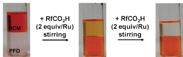
Fig. 2. Switch of partitioning induced by surfactant between a hydrocarbon (DCM = dichloromethane) and a fluororous phase (PFD = perfluorodecalin). A complex is formed between the red dye [Ru(bipy)_3]^{2+} ( Ru = ruthenium, bipy = bipyridine) and the perfluoropolyether carboxylic acid RfCOOH leading to the extraction of the ruthenium through complexation in the fluororous phase. Reprinted from Correa et al. [88], with permission of The Royal Society of Chemistry.
