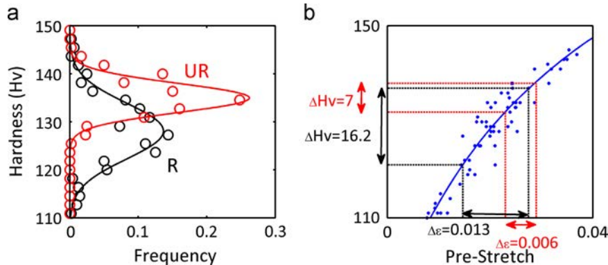
Fig. 4. (a) Hardness distributions measured on an UR and a R AA2198 specimens and (b) hardness as a function of pre-stretch after 7 h of heat treatment at 155 °C.
