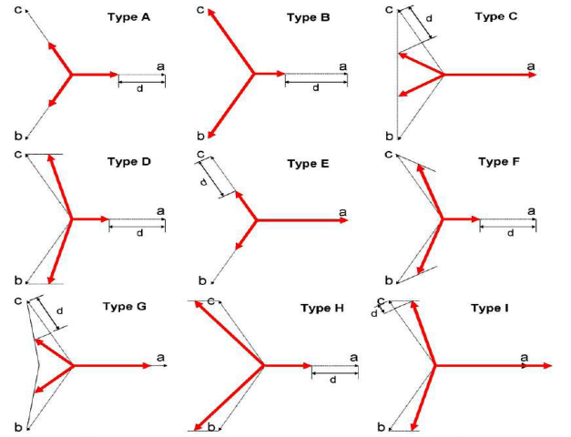
Fig. 4. Voltage sag main signatures [8].
