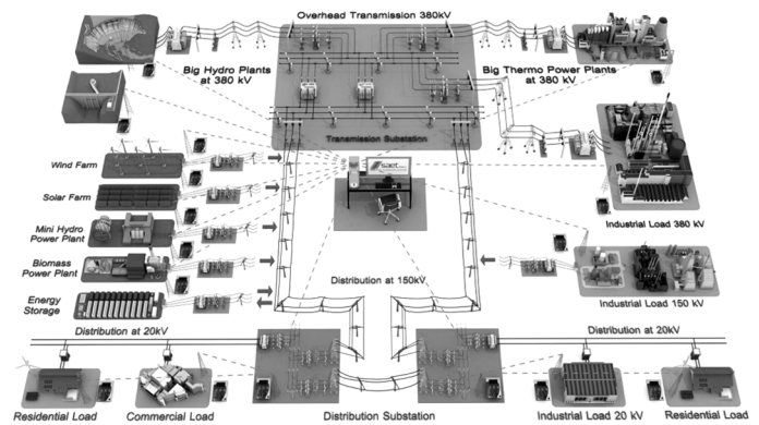
Fig. 1. A smart grid topology [© SAET].
