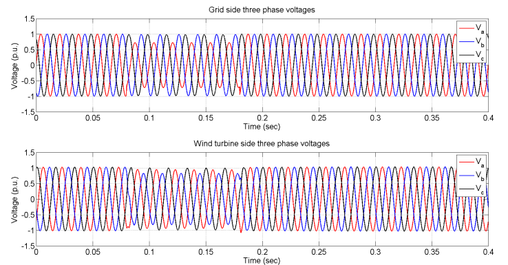
Fig. 7. Three phase voltages during a sag voltage in both sides of transmission line.
