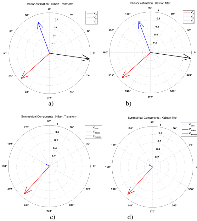
Fig. 8. Phasors representation and the corresponding symmetrical component.
