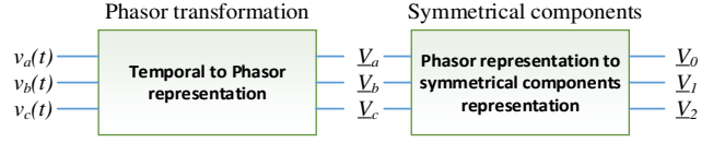
Fig. 5. Scheme for temporal to symmetrical components representation.
