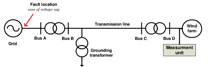
Fig. 6. Simulated system for voltage sag detection.
