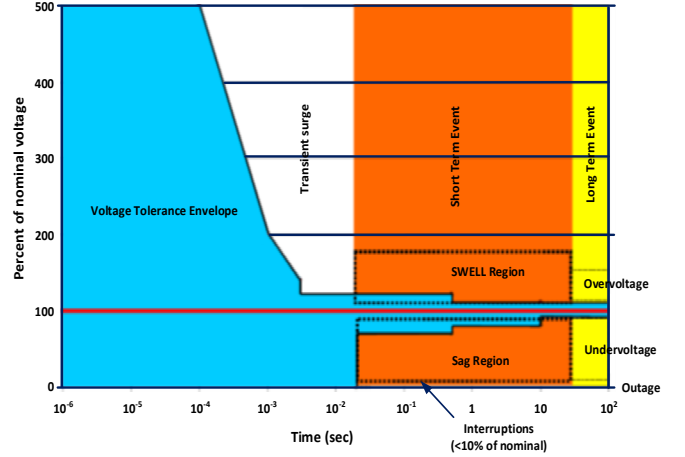
Fig. 3. Voltage events classification.
