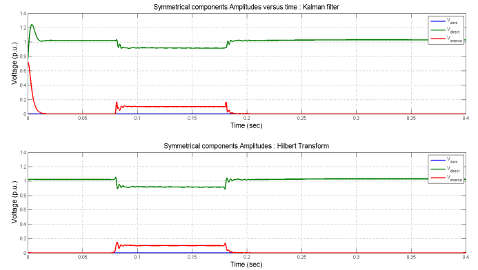
Fig.11. Amplitude variation of symmetrical components.
