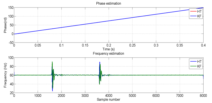
Fig.10. Instantaneous phases and frequency estimation.
