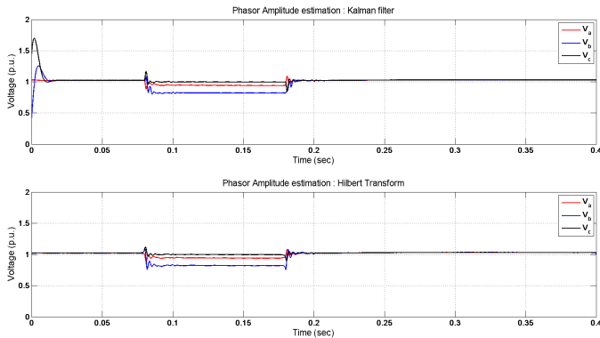
Fig.9. Amplitude variation of phasors.
