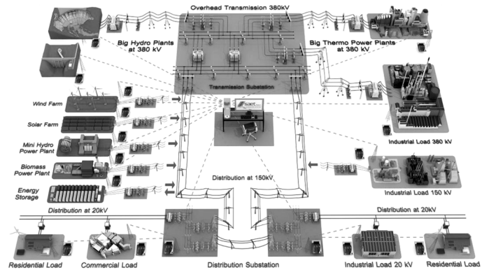
Fig. 1. A smart grid topology [© SAET].
