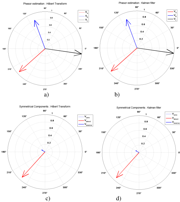
Fig. 8. Phasors representation and the corresponding symmetrical component.
