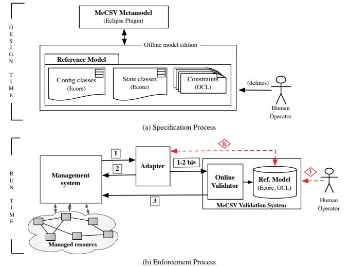
Fig. 2. Framework's Approach and Runtime Architecture
