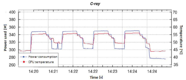
Fig. 2. C-ray power consumption and CPU temperature over time
