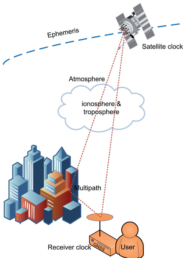
Figure 7 Error sources
