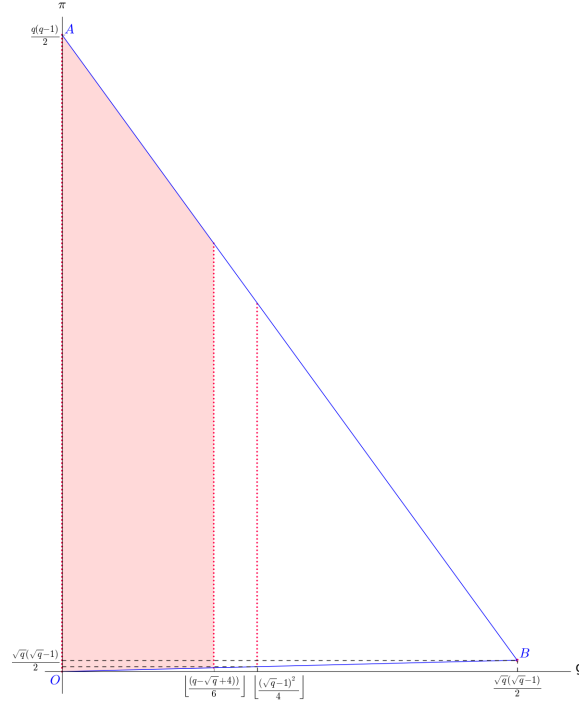
FIGURE 1. The set \Gamma_q is contained in the set of integers points inside the triangle (OAB) . The dots correspond to the couples (g, \pi) that we have proved to be in \Gamma_q . The rest of the set \Gamma_q has to be contained in the colored trapezoid.
