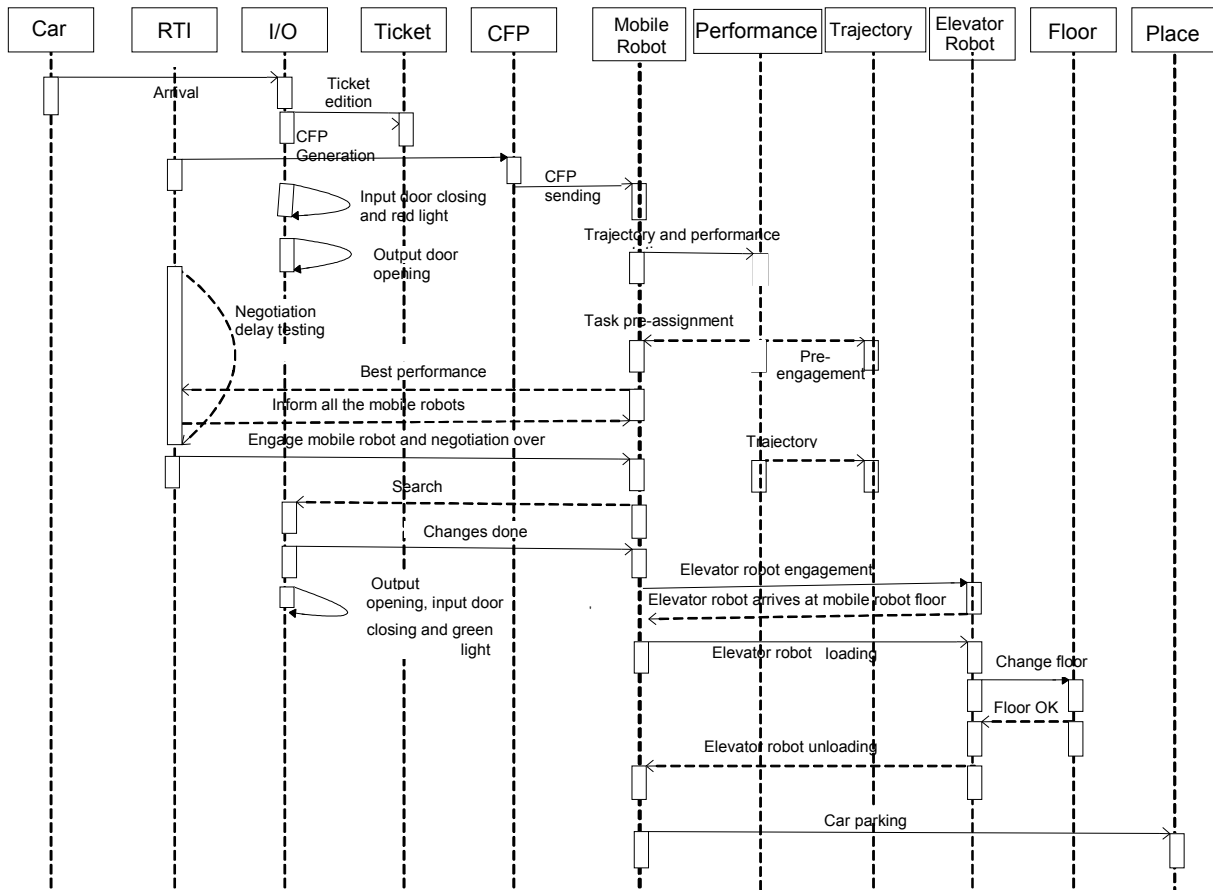
Figure 9: Sequence diagram
