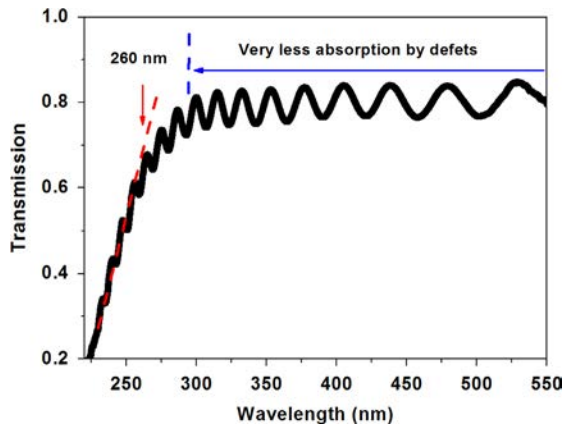
Fig. 7. Transmission spectrum at room temperature of 5-period AlN/BAlN heterostructure grown on AlN template.
