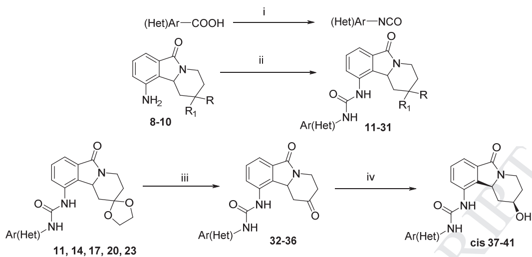
Scheme 3. Reagents and conditions : i) a) Et 3 N (1.3 eq.), -10 °C, THF, 5 min. ; b) ClCO 2 Et (1.5 eq.), -10 °C, THF, 2 h ; c) NaN 3 (1.7 eq.), -10 °C, H 2 O, 1 h ; d) toluene, reflux, 1 h ; ii) (Het)ArNCO, dioxane, 100 °C, 24 h ; iii) HCl 10%, acetone, reflux, 3 h ; iv) NaBH 4 (2.0 eq.), THF/MeOH (1/1), 0 °C-5 °C, 2 h. For yields see Table 1.
