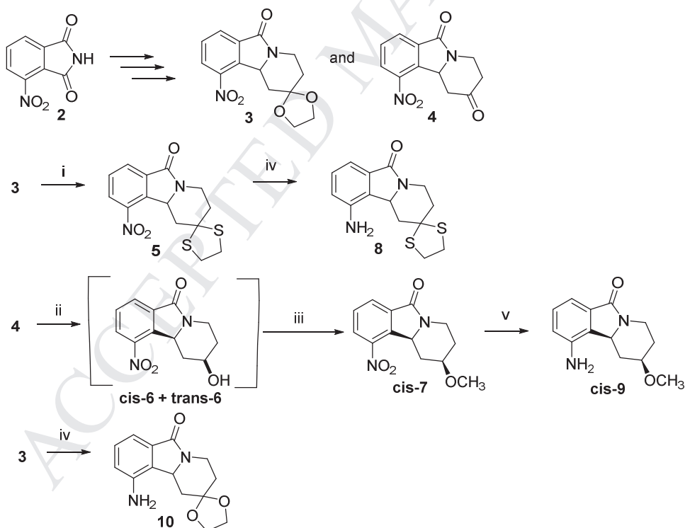
Scheme 2. Reagents and conditions : i ) 1,2-ethanedithiol (5.0 eq.), \text{BF}_3 \cdot \text{Et}_2\text{O} (5.0 eq.), \text{CH}_2\text{Cl}_2 , r.t., 24 h, 86% ; ii ) \text{NaBH}_4 (2.0 eq.), THF/MeOH (1/2), -20^\circ\text{C} to r.t., 5 h, 86% (mixture of cis-6 and trans-6 ) ; iii ) \text{Ag}_2\text{O} (4.0 eq.), \text{CH}_3\text{I} (10.0 eq.), THF, 50^\circ\text{C} , 48 h, 61% (from 4 ) ; iv ) \text{SnCl}_2 (15.0 eq.), EtOH, r.t., 12 h, 8 80% or 10 82% ; v ) \text{H}_2 , Patm, Raney Ni, EtOH, r.t., 14 h, 95%.
