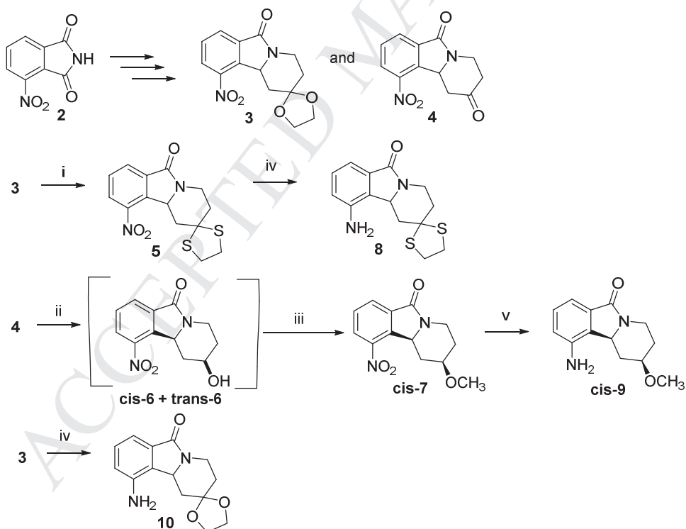
Scheme 2. Reagents and conditions : i ) 1,2-ethanedithiol (5.0 eq.), BF_3 \cdot Et_2O (5.0 eq.), CH_2Cl_2 , r.t., 24 h, 86% ; ii ) NaBH_4 (2.0 eq.), THF/MeOH (1/2), -20^\circ C to r.t., 5 h, 86% (mixture of cis-6 and trans-6 ) ; iii ) Ag_2O (4.0 eq.), CH_3I (10.0 eq.), THF, 50^\circ C , 48 h, 61% (from 4 ); iv ) SnCl_2 (15.0 eq.), EtOH, r.t., 12 h, 8 80% or 10 82% ; v ) H_2 , Patm, Raney Ni, EtOH, r.t., 14 h, 95%.
