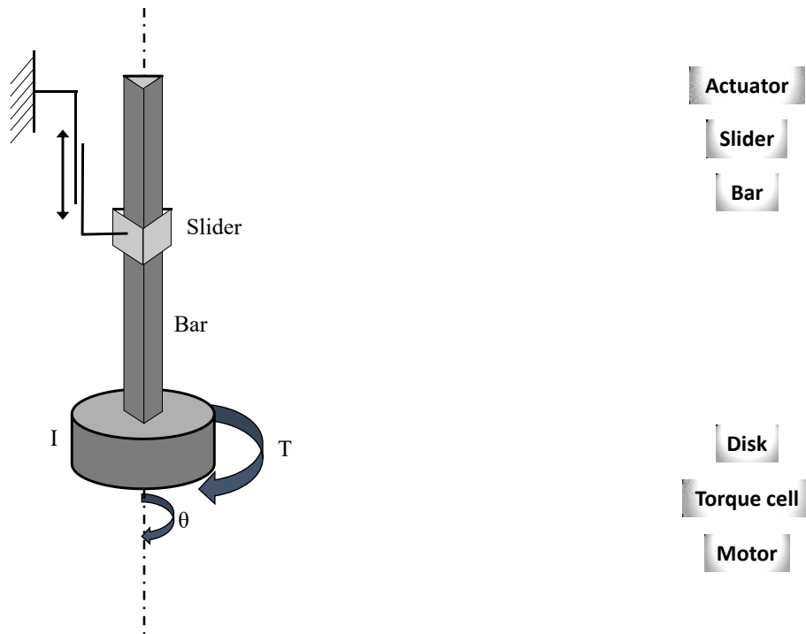
Fig.1: Experimental mounting of the prism beam in torsion and its representative scheme on left.
