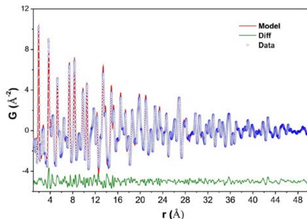
Figure 7. Refinement of the PDF of the phase prepared by thermal decomposition of \text{FeF}_3 \cdot 3\text{H}_2\text{O} decomposed at 130^\circ\text{C} under self-generated atmosphere.
