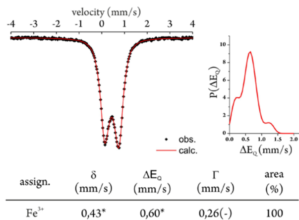
Figure 8. ^{57}\text{Fe} Mössbauer spectra of HTB- \text{FeF}_{3-x}(\text{OH})_x hydroxyfluoride. Right panel: Quadrupole splitting distributions. ^{57}\text{Fe} Mossbauer parameters obtained from the reconstruction of spectra shown in left. * Average value
