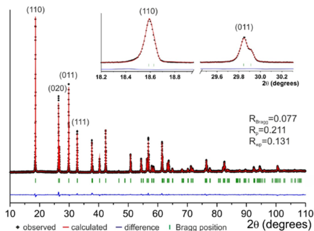
Figure 1. Rietveld refinement of the x-ray diffraction pattern (CoK \alpha source) of FeF 3 ·3H 2 O.
