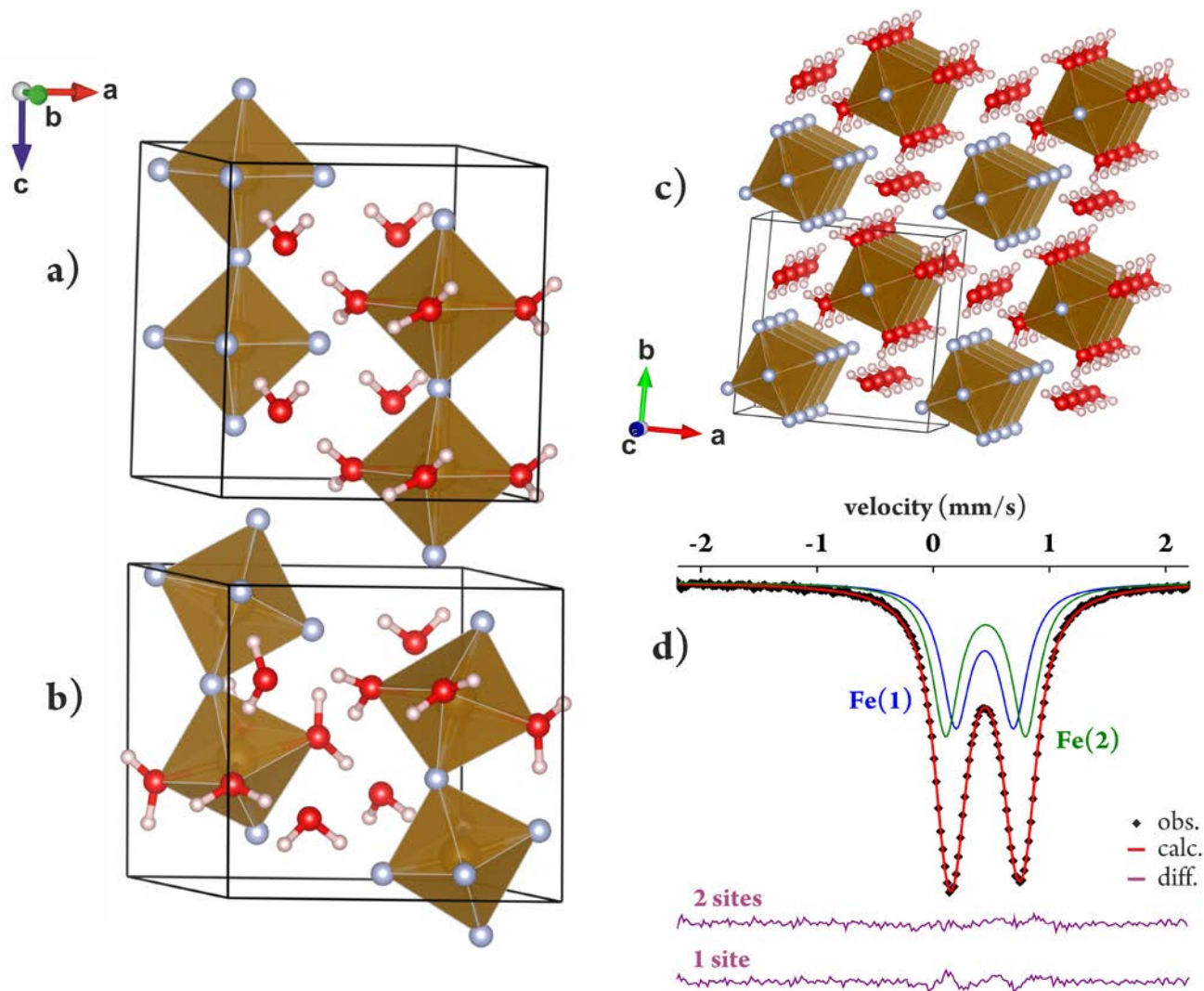
Figure 3. a) 1 \times 1 \times 2 supercell of the lowest energy configuration (configuration 1). b) Supercell with alternating FeF 6 and FeF 2 (H 2 O) 4 octahedra along the c-axis. c) Extended cell of the lowest energy configuration. d) Mössbauer spectrum of \beta -FeF 3 ·3H 2 O reconstructed using two Fe 3+ signals, Fe(1) (blue) and Fe(2) (green). The difference between the observed and calculated values is represented as violet lines.
