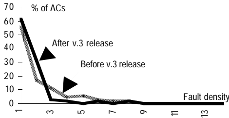
Figure 5 - Fault density distribution among ACs
