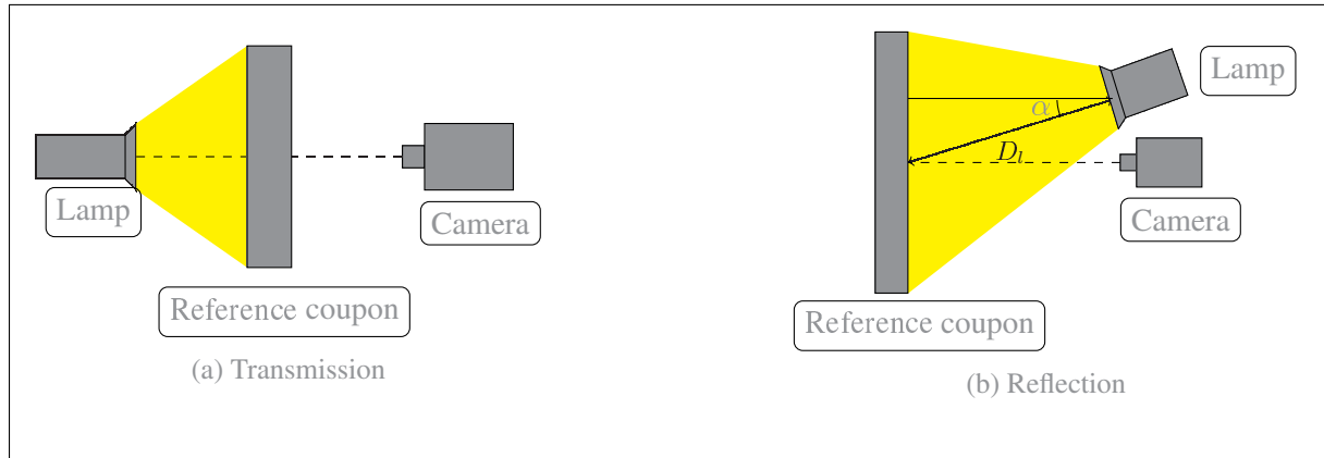
Figure 2: Infrared thermography setups
