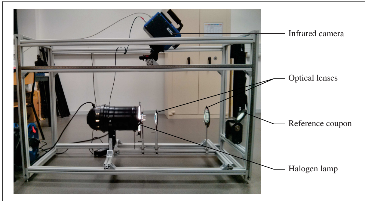
Figure 5: Test bench
