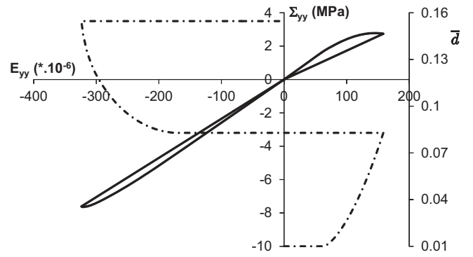
Fig. 14. Simulation of tensile loading followed by unloading and reloading in compression for axis loading ( \psi = 0^\circ ) (full line: axial stress-strain curve \Sigma_{yy}-E_{yy} ; dashed line: evolution of mean damage \bar{d} with axial strain).
