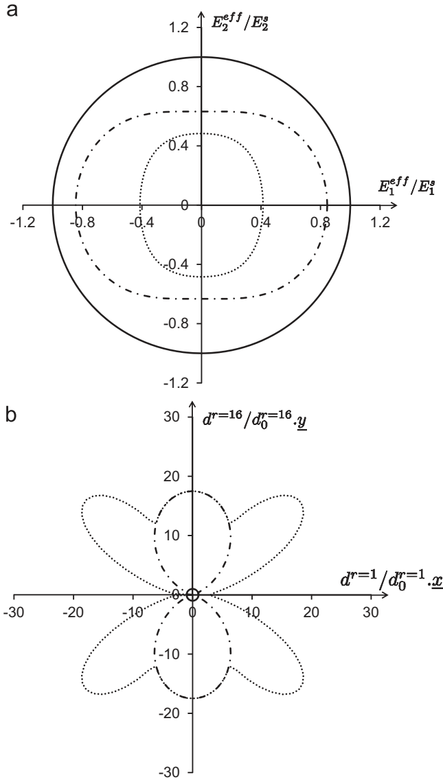
Fig. 16. Evolution of (a) the distribution of the normalized effective Young modulus E_2^{eff}(\underline{\nu})/E_2^s(\underline{\nu}) and (b) the distribution of the normalized damage d^r/d_0^r after tensile loading (dash lines) and compression reloading (dot lines) (full lines refer to initial states – unit circles).
