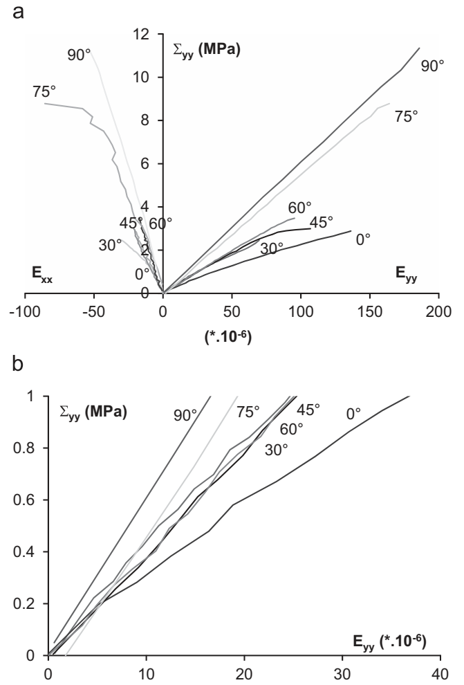
Fig. 7. Experimental stress-strain responses for different loading orientations \psi = 0^\circ, 30^\circ, 45^\circ, 60^\circ, 75^\circ, 90^\circ ( \Sigma_{yy} the axial stress, E_{yy} the axial strain, E_{xx} the radial strain): (a) global response, (b) zoom on linear elastic part.
