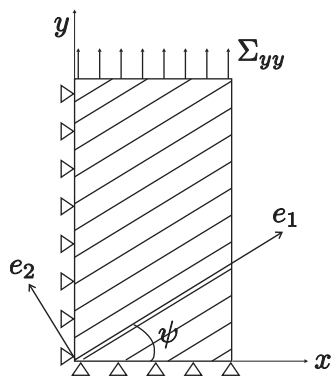
Fig. 6. Uniaxial tensile test and anisotropy orientation.
