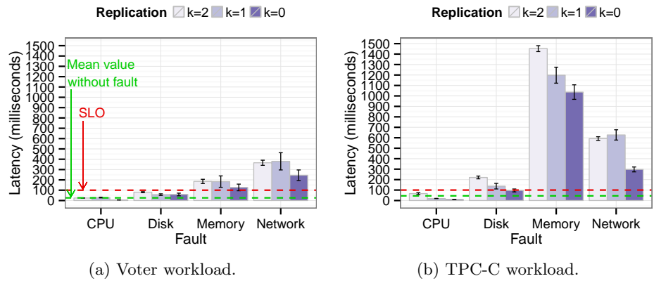
Fig. 5: Medium fault impact on VoltDB with different k values.
