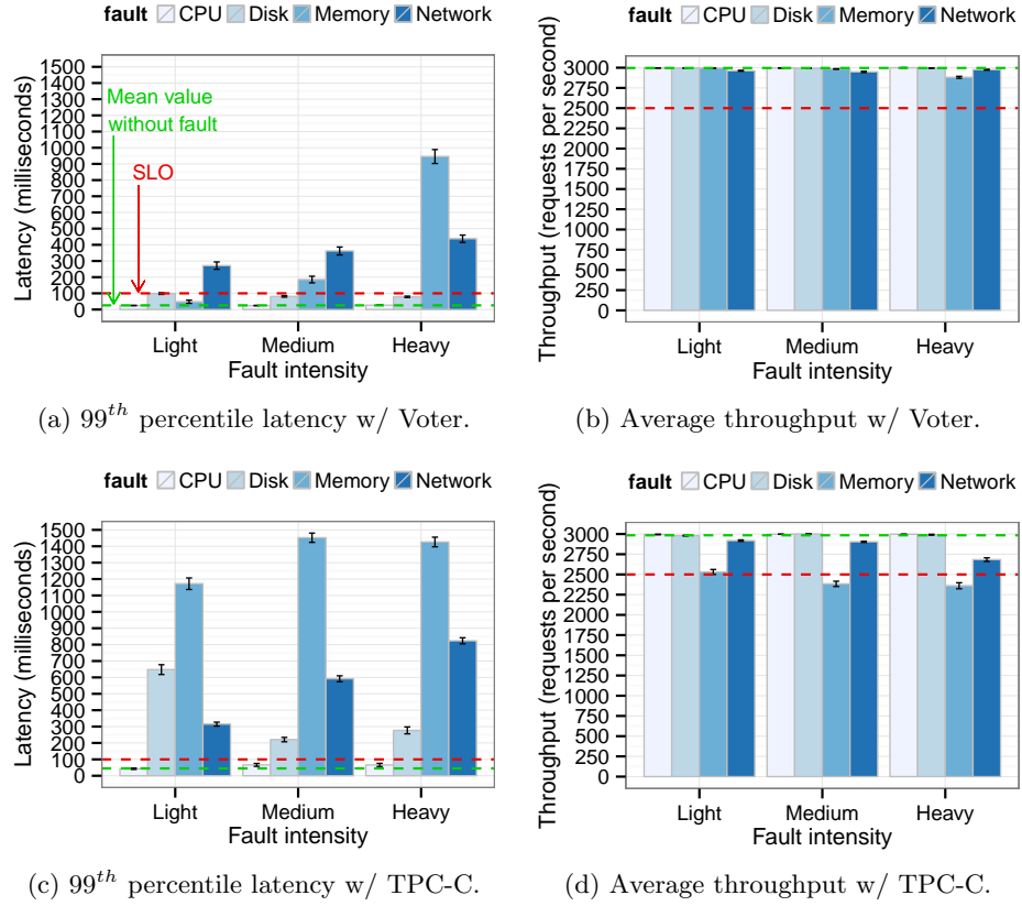
Fig. 4: Performance anomalies in VoltDB as serving Voter and TPC-C, with a replication degree k=2 .
