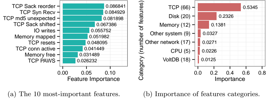
Fig. 6: Analysis of the importance of features for anomaly detection.
