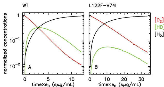
Fig. 4 Isotope-exchange assay (eqn (22)) of the WT form (A) and L122F-V74I mutant (B) of Desulfovibrio fructosovorans [NiFe]-hydrogenase. The changes in concentrations of \text{D}_2 , \text{HD} and \text{H}_2 are used to determine the rate of H 2 exit from the enzyme. 63,135 e_0 is the concentration of enzyme. That the mutant produces less HD than the WT enzyme indicates that the mutation slows diffusion along the gas channel. Figure reproduced from ref. 63 (copyright 2012 American Chemical Society).
