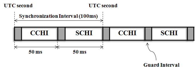
Fig. 3: Network synchronization
