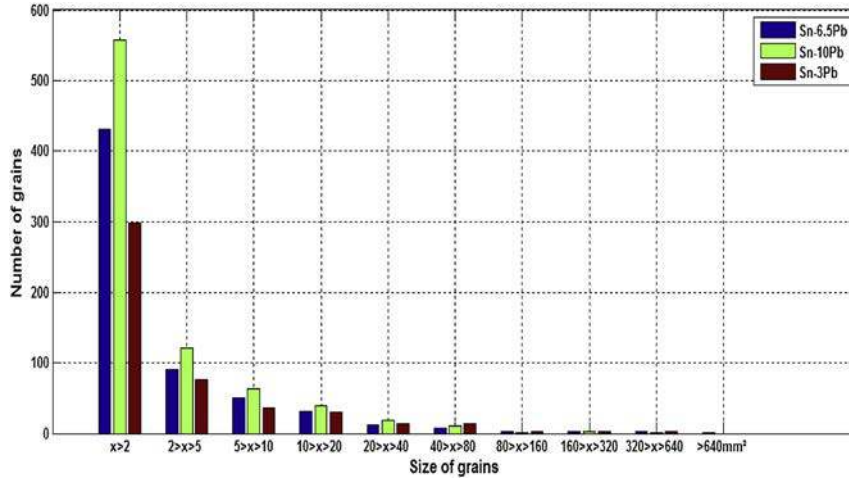
Fig. 11. Distribution of grain size for the three samples: Sn–3 wt.%Pb, Sn–6.5 wt.%Pb and Sn–10 wt.%Pb alloy. Experimental conditions are: \Delta T = 40 K, CR = 0.03 K/s.
