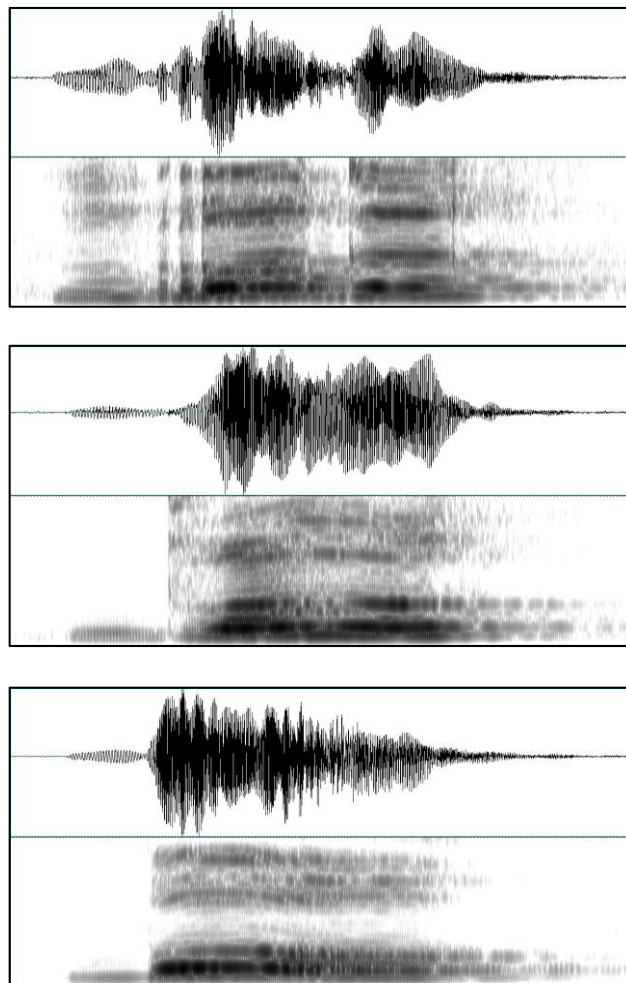
Figure 1: Waveforms and spectrograms of [mb́ógé] ‘fire’, [b̥b́óŋé] ‘poverty’, and [b̀òò] ‘two’.
