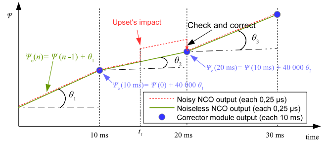
Fig. 5. Correction of errors in RvC method; when an error occurs at time step t_i , it can be corrected at time at 20 ms thanks to the correct output of the correction module.
