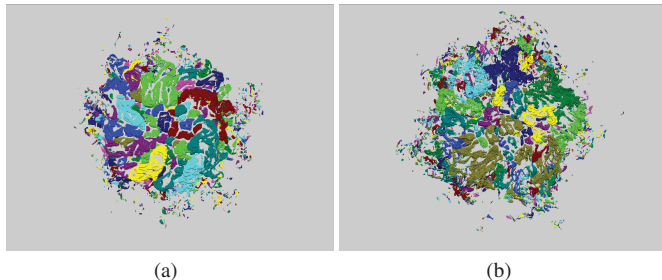
Fig. 12. (a) Burning cells in the SwirlH2 data at time step 1500 using a fuel consumption threshold of 8.0 \text{ kgH}_2/\text{m}^3 \text{ s} ; (b) Burning cells in the SwirlH2Fast data at threshold 12.0 \text{ kgH}_2/\text{m}^3 \text{ s} .
