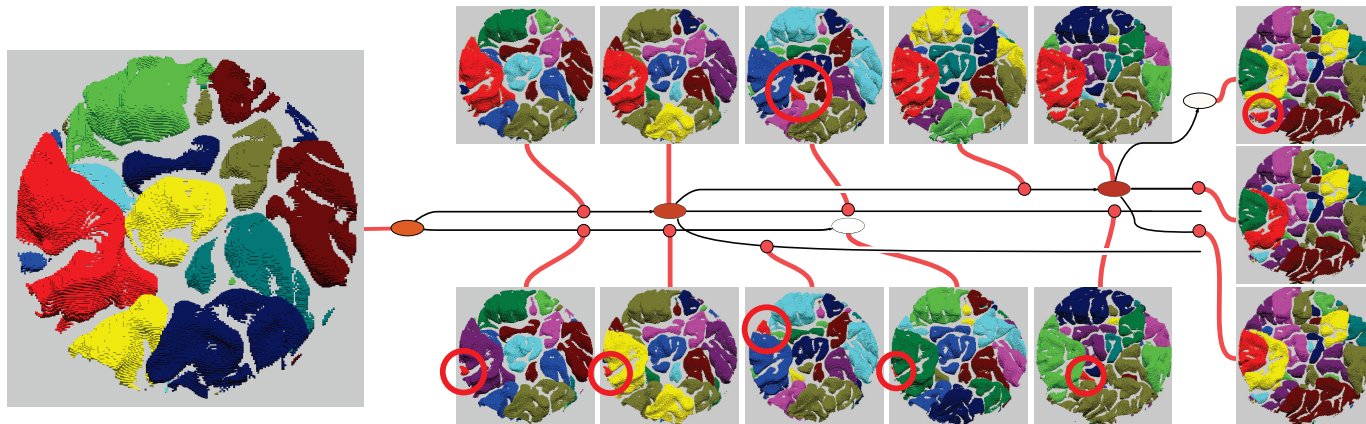
Fig. 7. Example of burning cells being tracked over time. The graph shows a small portion of the tracking graph for the SwirlH2 data set between time steps 1420 through 1465. The insets show the corresponding segmentation as nodes are selected in the graph. Over the course of these time steps the large cell represented by the left most node slowly sheds smaller cells until it finally breaks apart into three independent pieces.
