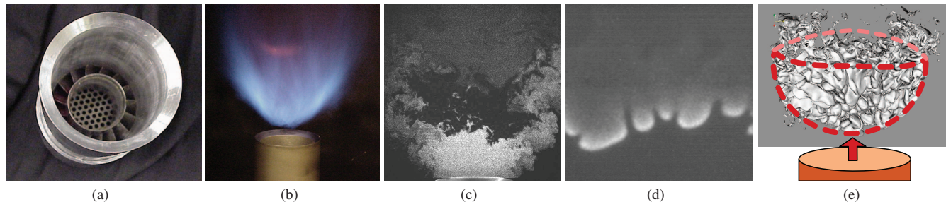
Fig. 1. (a) Photo of a typical laboratory low-swirl nozzle. (b) Photo of a lean premixed \text{CH}_4 low-swirl flame. (c) Experimental Mie scattering image of a lean premixed \text{H}_2 flame. (d) PLIF data imaging the OH concentration in a lean premixed \text{H}_2 flame. (e) Rendering of the burning cells of the SwirlH2 simulation data. The cells form a bowl shaped structure with the arrow indicating the direction of the fuel stream.
