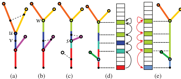
Fig. 6. Two-pass segmentation corresponding to a merge tree with critical points colored according to the branches they represent: (a) An initial tree segmented into branches indicated by color; (b) Adding the dotted edge shown in (a) results in a partial merge of branches causing the blue saddle u to become regular and a new green saddle w to appear; (c),(d) Adding further edges creates and destroys additional critical points as well as the corresponding segments. Note that labels are updated only as a side-effect of necessary merge-sorts and thus incur virtually no additional computational cost; (d) Using the indices of critical points as labels, the labels form linked lists of vertices terminating in a critical point, representing the head of a linked list; (e) Traversing the implicit linked list backward while traversing the merge graph (containing only critical points) allows one to correct all labels along the path.
