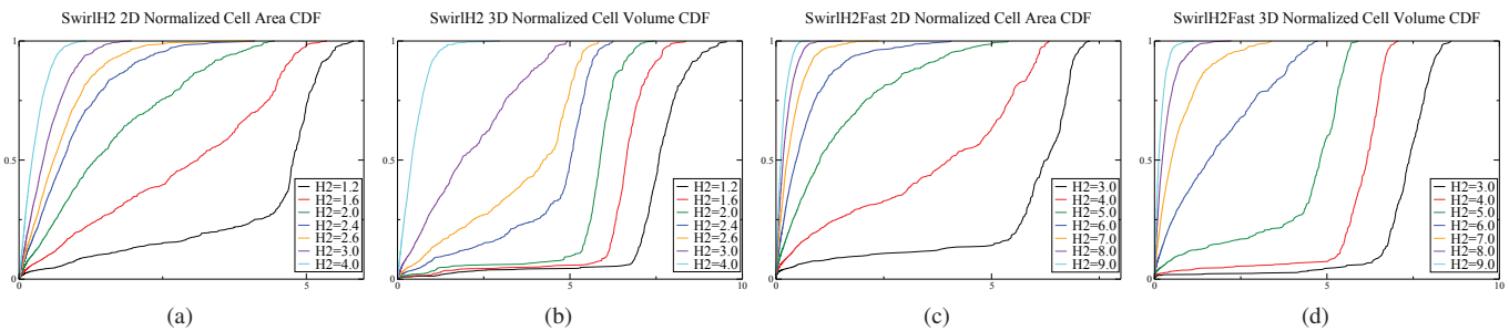
Fig. 15. Weighted cumulative density functions of the distributions of cell sizes for various thresholds for the surface based analysis of [6] (a),(c) and the volumetric analysis presented here (b),(d) for the SwirlH2 and SwirlH2Fast data set respectively. Unlike the idealized flames of [64] the distributions for lower thresholds are exponential indicating few large cells rather than the expected many small cells.
