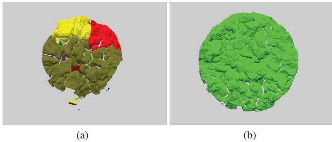
Fig. 10. Burning cells within a cylinder of radius 2.5cm centered in the middle of the data using 2.6kg_{H_2}/m^3s as fuel consumption cut-off. The view direction is in the direction of the fuel stream. (a) Time step 1500 of the SwirlH2 data; (b) Time step 3000 of the SwirlH2Fast data.
