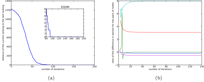
Figure 1: Experiments validating conjectures 1 and 2. The experiments are carried out on the symmetrized polblogs network \mathcal{G} , a network of 1222 nodes and 16717 edges. Figure ?? validates conjecture 1 by comparing the ranking of nodes according to their opinions to the ranking according to the last opinions obtained (for 200 iterations). As we can see, after only 95 iterations the ranking is not changing. The distance between the ranking we used is simply the number of misclassified nodes. Figure ?? validates conjecture 2 by plotting the ratio of the difference of two randomly chosen pairs of nodes. The experiment has been made 5 times, there are therefore five curves. As we can see, after only 40 iterations the ratio is quite constant, thus the differences in the opinion of a given pair of nodes is proportional to the one of any other pair.
