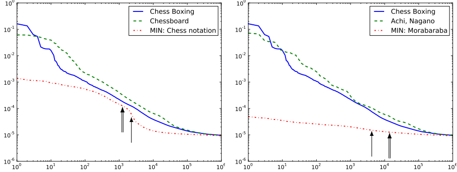
Figure 13: Each figure shows the curves corresponding to a trial: the y axis represents the scores and the x axis represents the ranking of the nodes according to their scores. The first (resp. second) curve is the carryover opinion run from the node Chess Boxing (resp. a candidate for v , the legend shows the label of the candidate), while the third curve shows the minimum, the label of the first ranked node is in the legend. The first trial is successful, while the second is not (no plateau/decrease structure). The double arrow shows the position of the “Chess Boxing” node, while the simple arrow shows the position of the sharpest slope.
